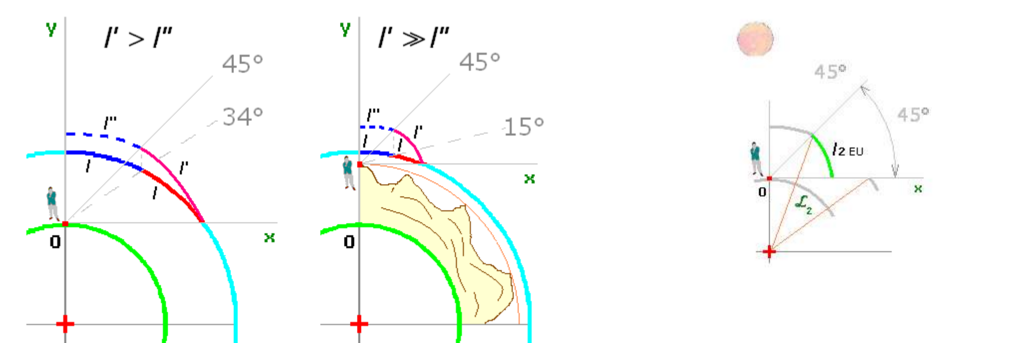
Obr. 4. 27 zvetseni-Mesice-hory
